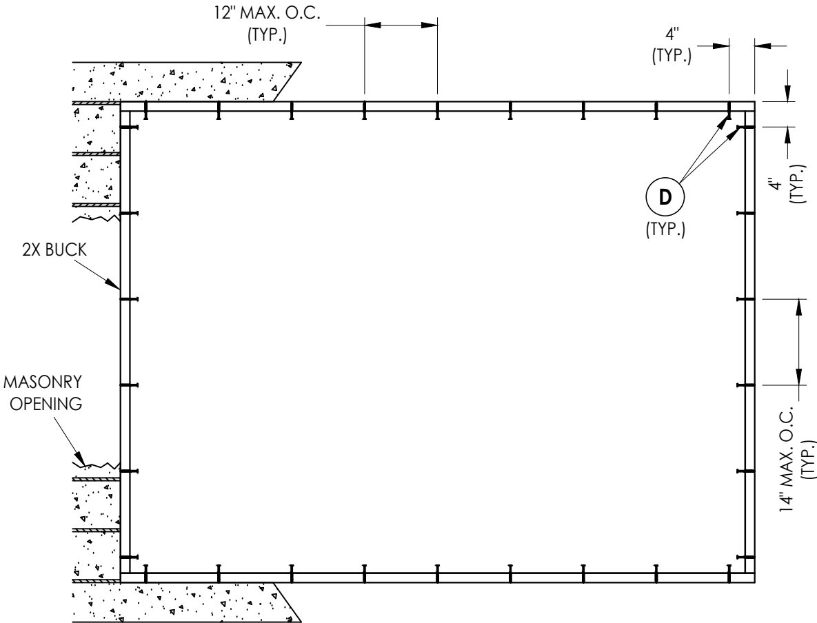
BUCK ANCHORING 96" X 72" MAX.
