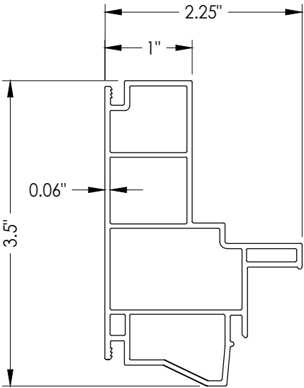
1 FRAME (5400 Series)
